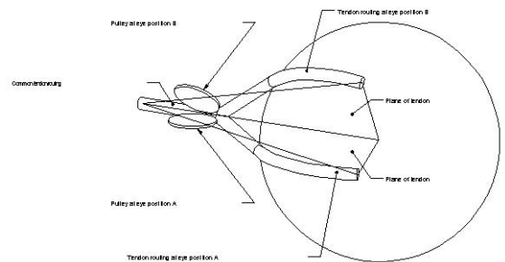
Fig. 9. Sketch of the tendon's paths, showing the tilting of the routing pulley (tendons and pulleys diameters not to scale).
