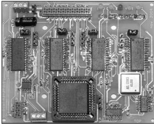
Fig. 15. The embedded real-time controller. The board has dimensions of 69 \times 85mm^2 to be integrated with the eye
