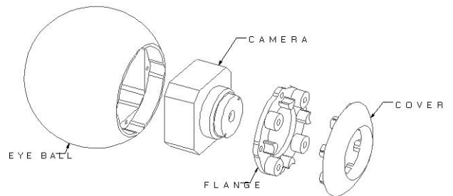
Fig. 5. Exploded view of the eye-ball (internal camera support spring not shown)
