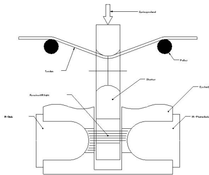
Fig. 14. Sketch of the tension sensor (not to scale).
