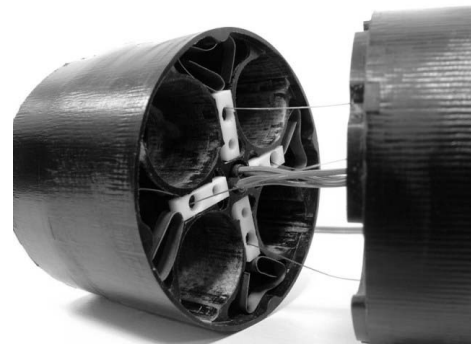
Fig. 13. Implementation of the embedded tendons' tension sensors. The picture shows the shutter and the spring, cables and tendons.
