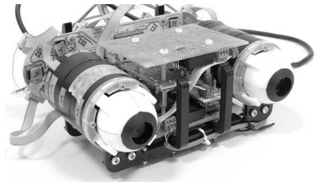
Fig. 16. Complete stereoscopic robot system
