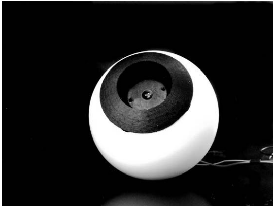
Fig. 6. Assembled eye-ball (camera cables shown in background)
